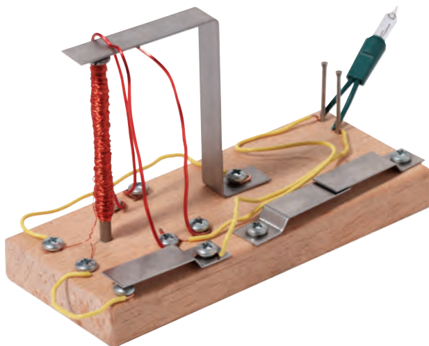
Electromagnet Kit
