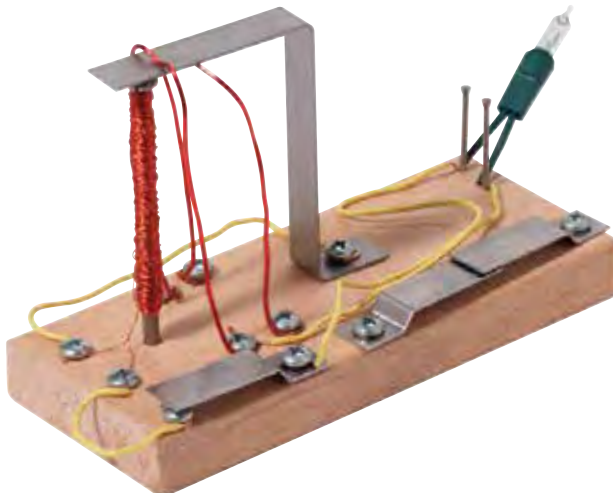
Electromagnet Kit
